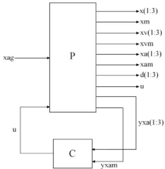
Figure 2: Control Structure
